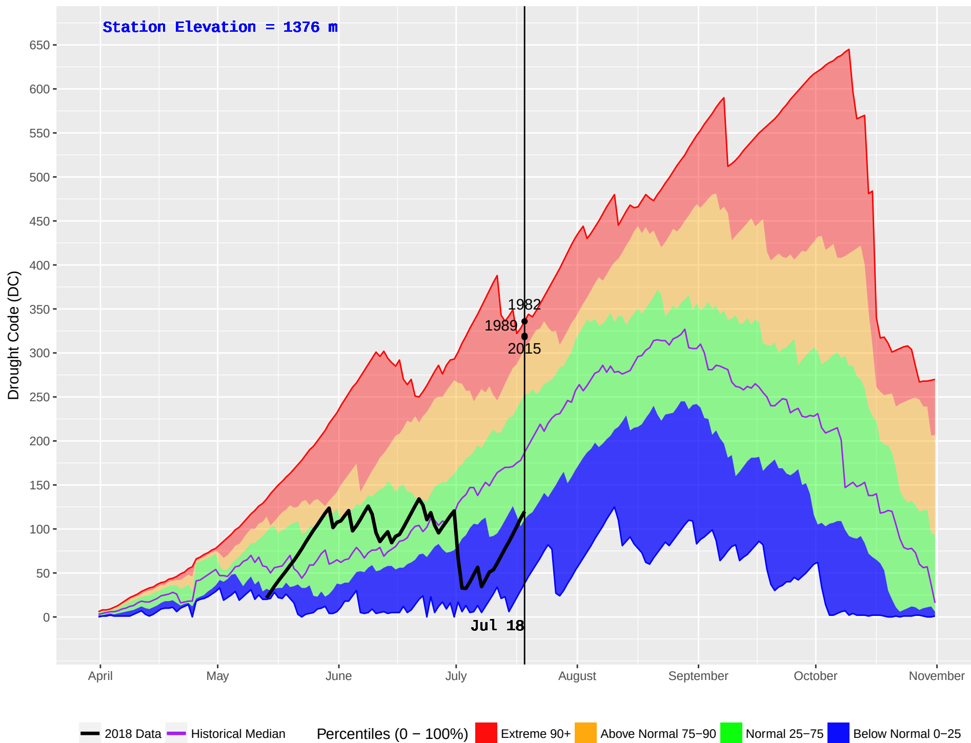
DUNCAN (385) : Historical (1981–2016) and Current (2018) Daily Drought Code (DC)
